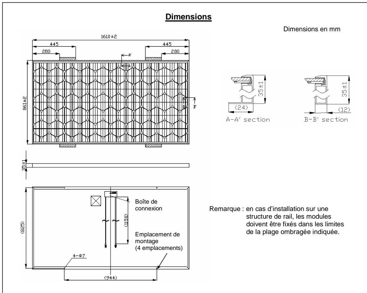
Figure 2-1: Dimensions
