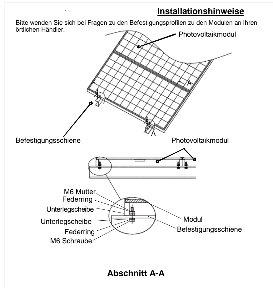
Abb. 1: Installation
